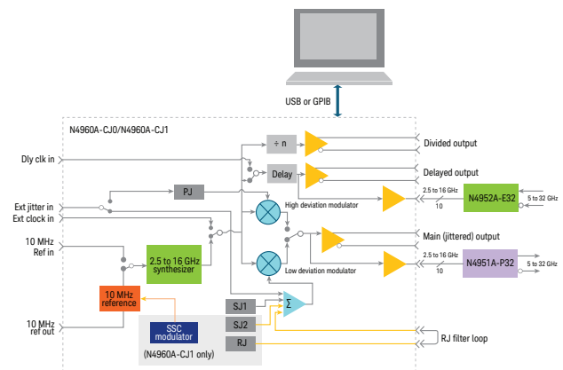
Block diagram (32 Gb/s system)
