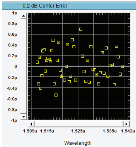
Less than \pm 1 pm deviation of the measured center wavelengths from the known values (according to NIST SRM 2517a) acquired at 200 nm/s sweep speed
